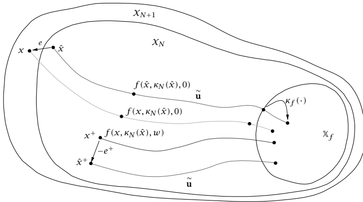
Figure 4.6: Although the nominal trajectory from \hat{x} may terminate on the boundary of \mathbb{X}_f , the three perturbed trajectories, including the one from \hat{x}^+ , terminate in \mathbb{X}_f . After Allan et al. (2017).
