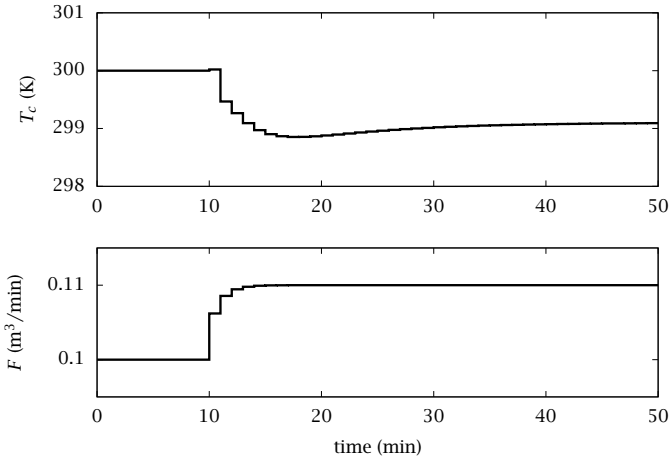
Figure 1.9: Two manipulated inputs versus time after a step change in inlet flowrate at 10 minutes; n_d = 2 .
