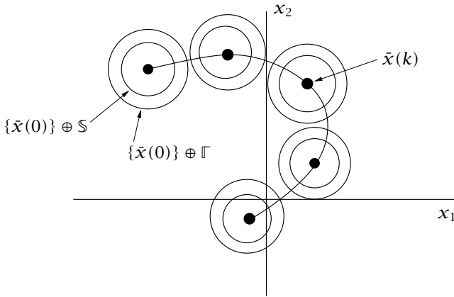
Figure 5.2: The system with disturbance. The state estimate lies in the inner tube, and the state lies in the outer tube.
