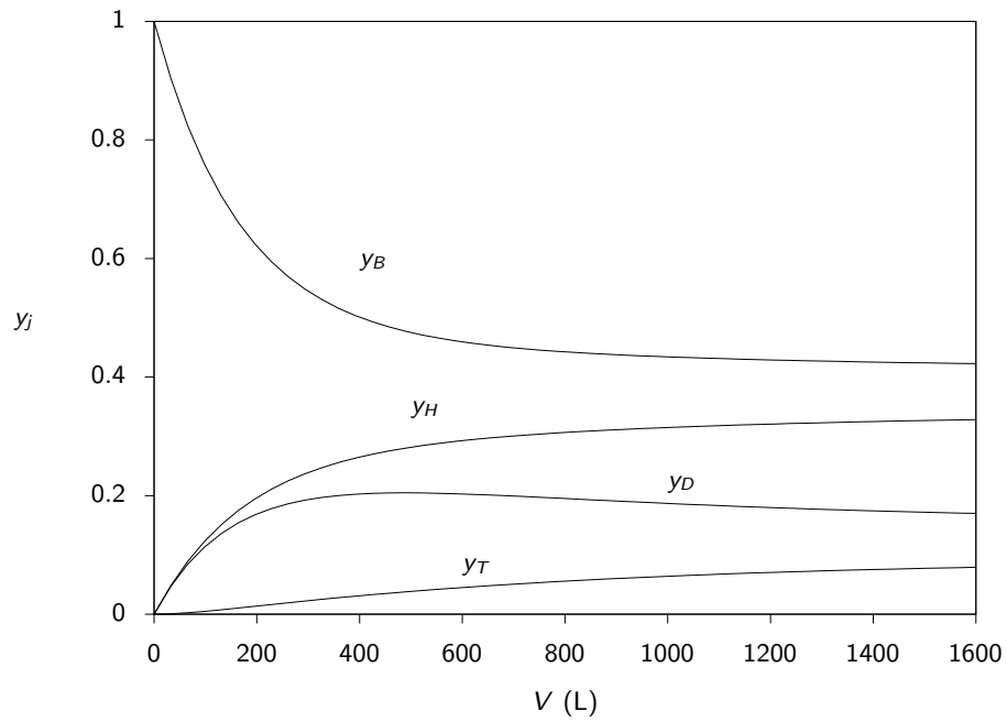
Figure 4.21: Component mole fractions versus reactor volume.
