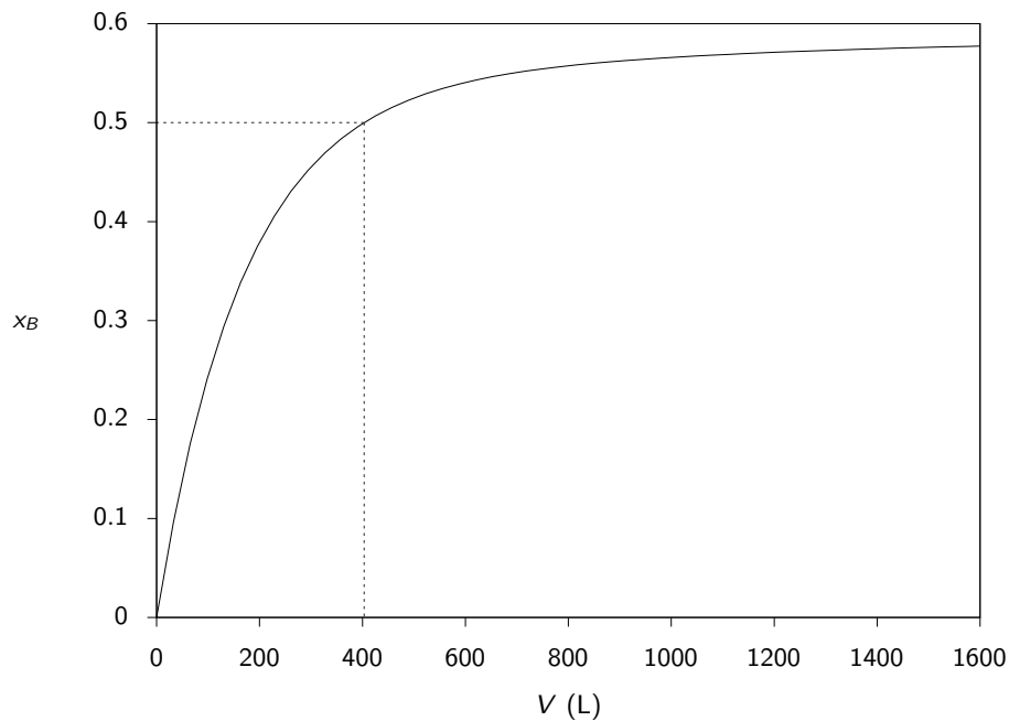
Figure 4.20: Benzene conversion versus reactor volume.
