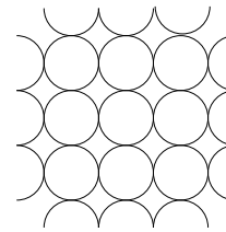
fcc (100)
