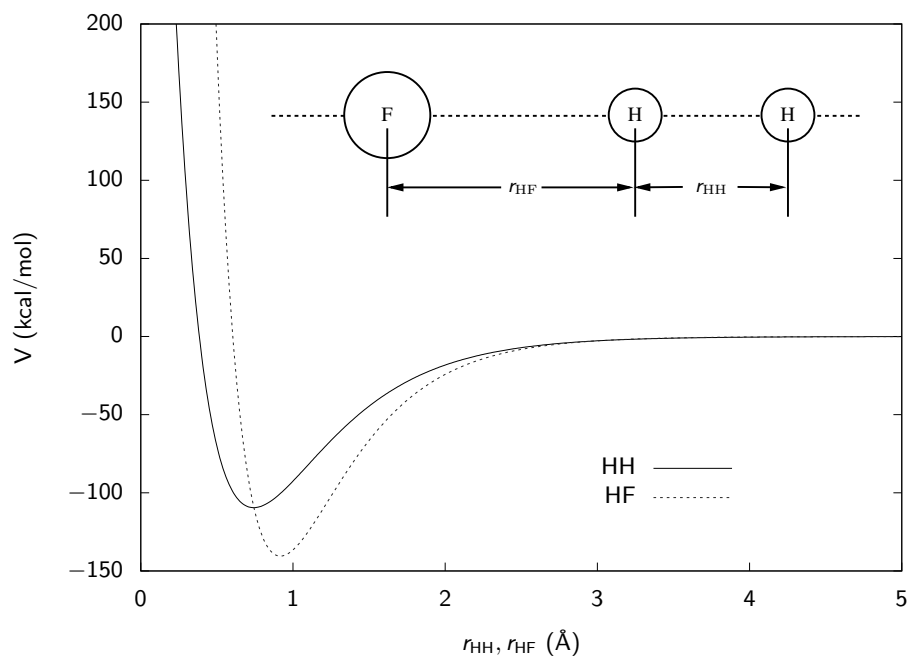
Figure 5.1: Morse potential for H 2 and HF.
