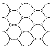
fcc (111)
