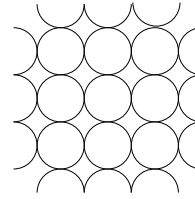
fcc (100)
