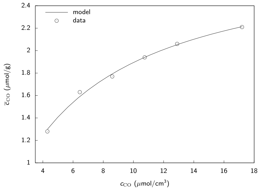
Figure 5.19: Langmuir isotherm for CO uptake on Ru.
