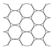
fcc (111)
