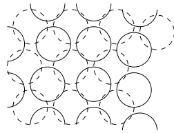
bcc (100)
