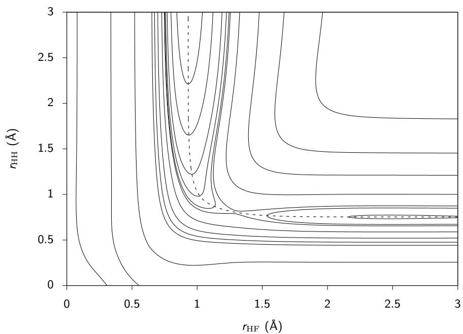
Figure 5.3: Contour representation of the potential-energy surface.
