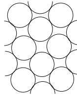
bcc (110)
