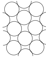
bcc (110)
