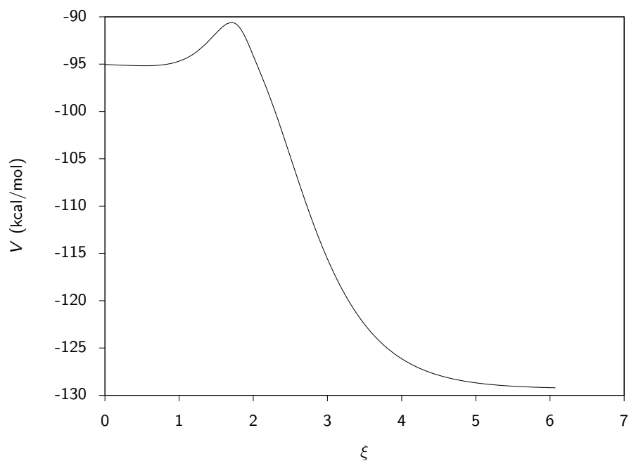
Figure 5.4: Reaction-coordinate diagram.
