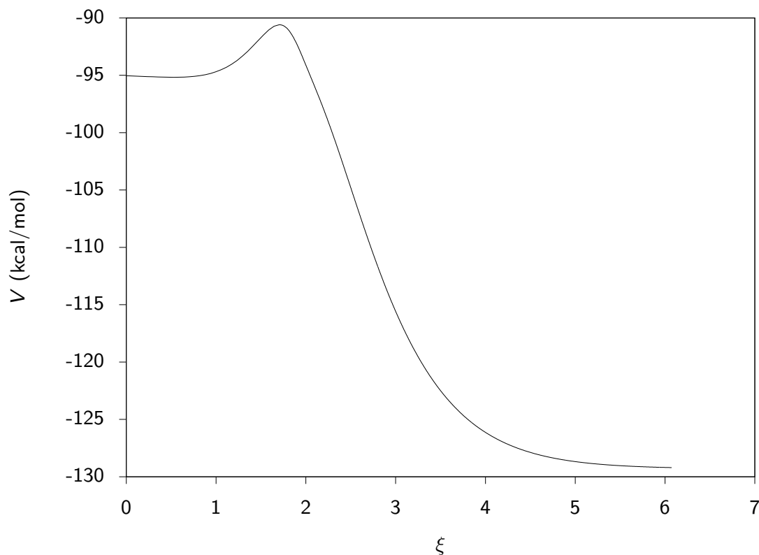
Figure 5.4: Reaction-coordinate diagram.
