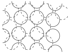
bcc (100)
