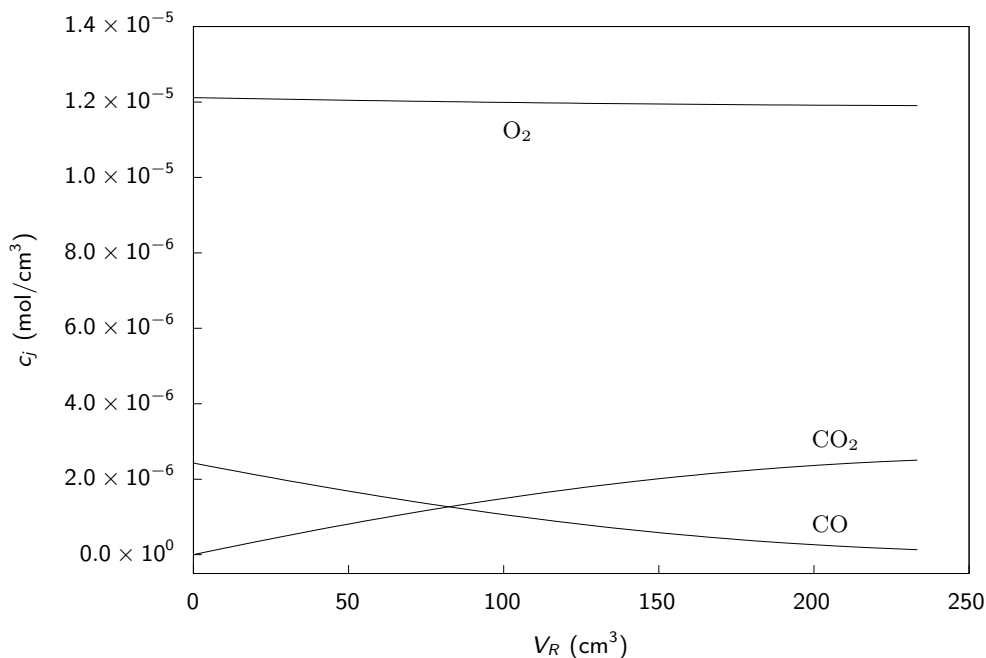
Figure 7.27: Molar concentrations versus reactor volume.
