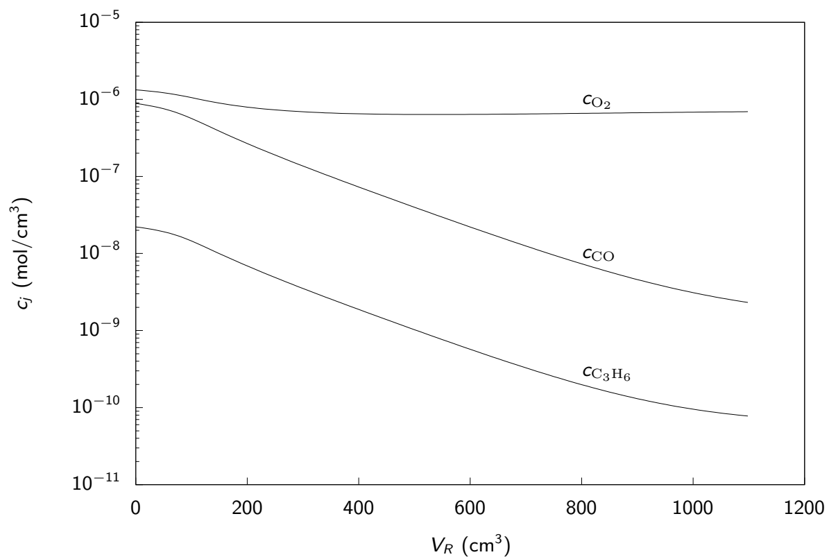
Figure 7.29: Fluid molar concentrations versus reactor volume.
