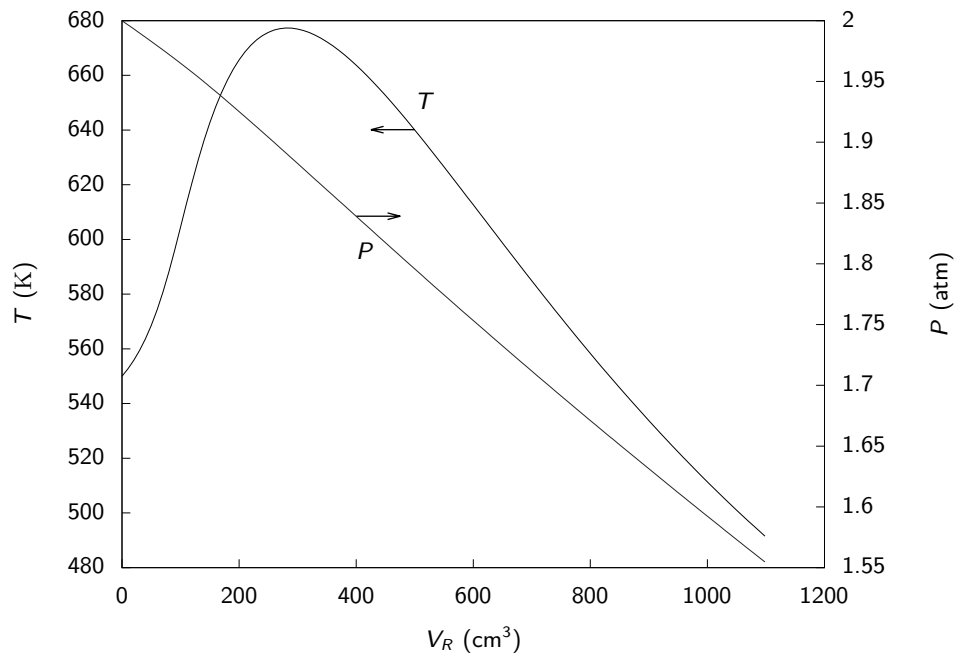
Figure 7.30: Fluid temperature and pressure versus reactor volume.
