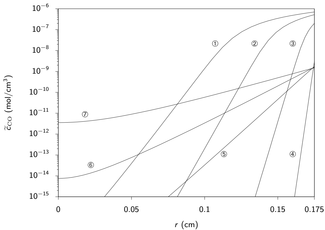
Figure 7.32: Pellet CO profiles at several reactor positions.
