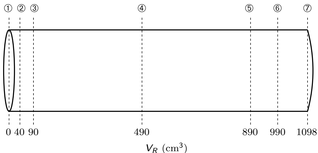
Figure 7.31: Reactor positions for pellet profiles.
