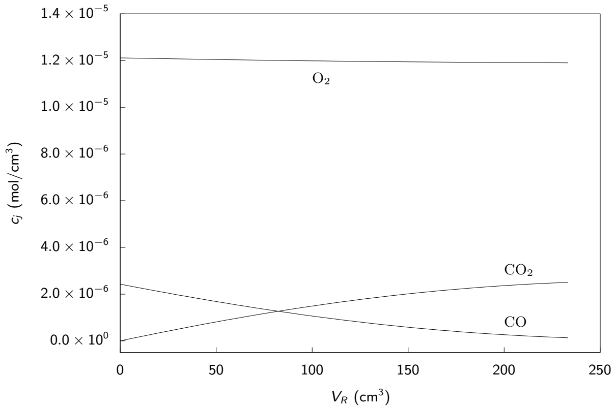
Figure 7.27: Molar concentrations versus reactor volume.
