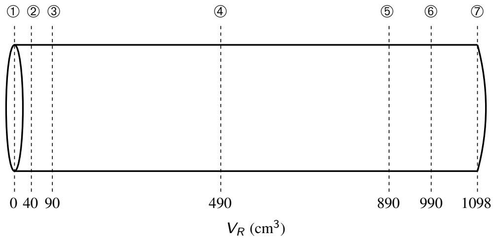
Figure 7.31: Reactor positions for pellet profiles.
