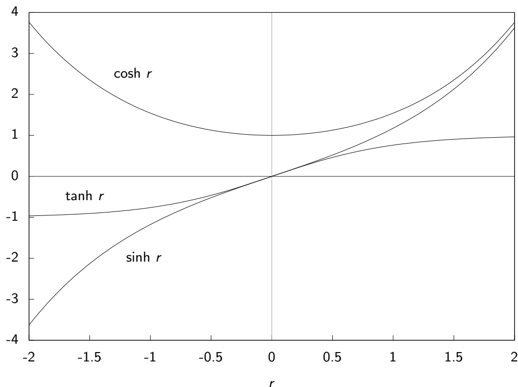
Figure 7.3: Hyperbolic trigonometric functions \sinh , \cosh and \tanh .
