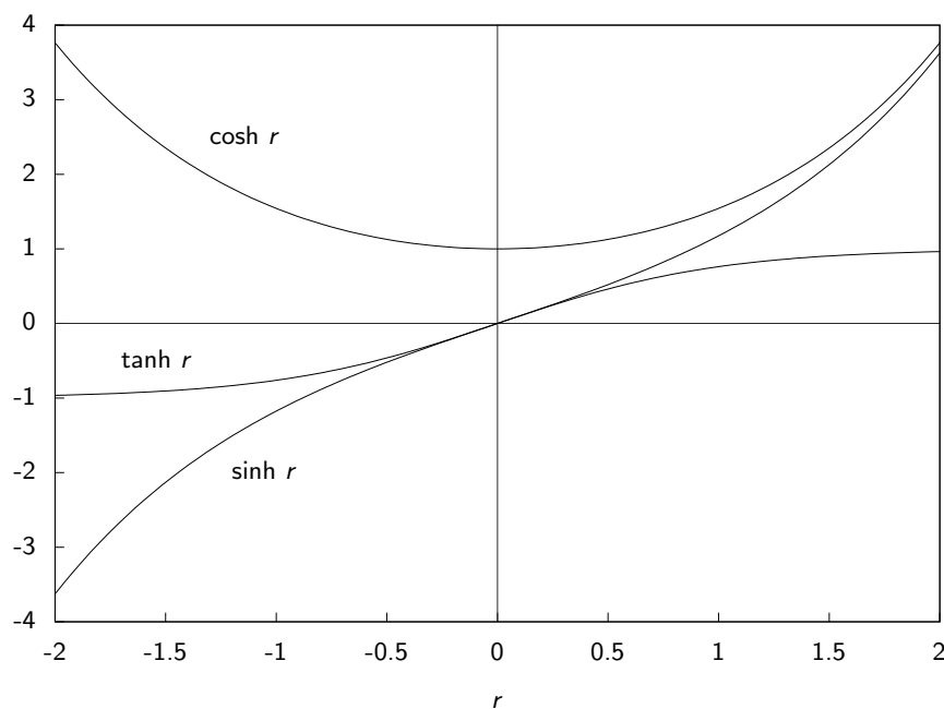
Figure 7.3: Hyperbolic trigonometric functions \sinh , \cosh and \tanh .
