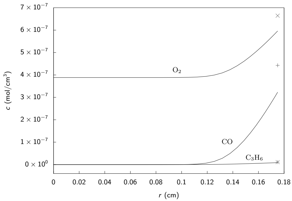
Figure 7.22: Concentration profiles of reactants; fluid concentration of O_2 ( \times ), CO ( + ), C_3H_6 ( * ).
