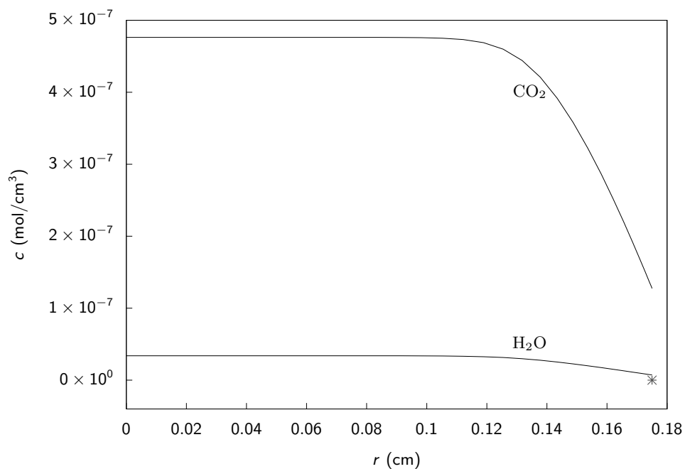
Figure 7.24: Concentration profiles of the products; fluid concentration of CO_2 ( \times ), H_2O ( + ).
