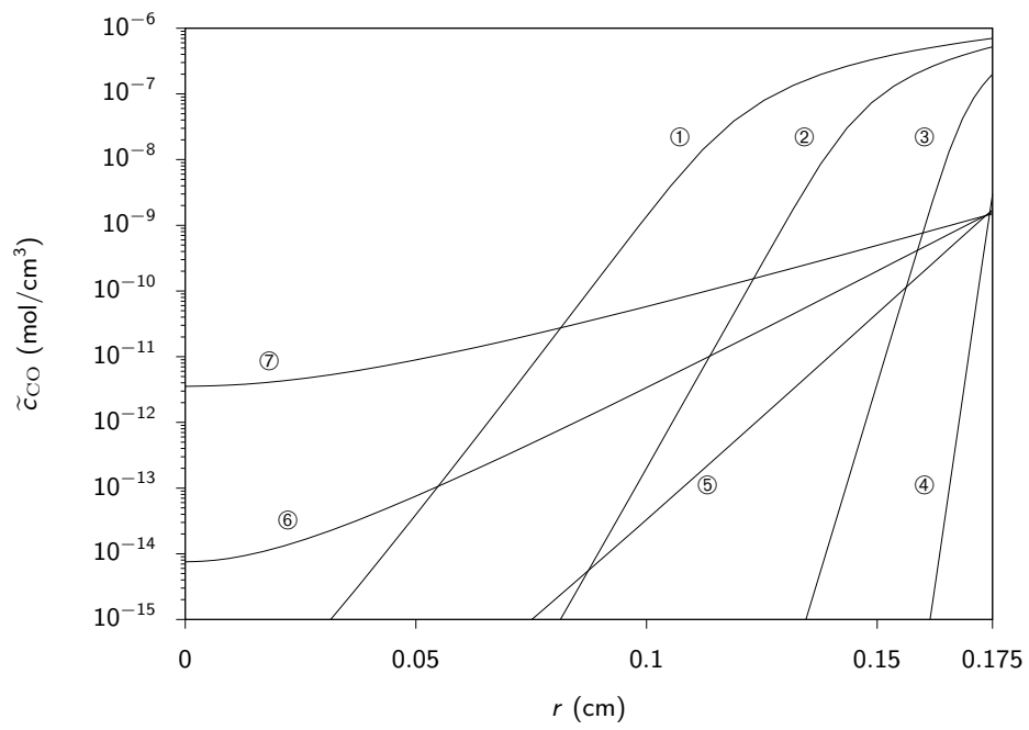
Figure 7.32: Pellet CO profiles at several reactor positions.
