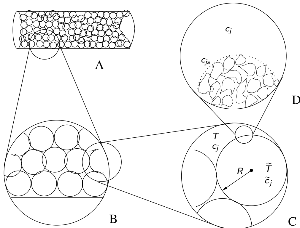
Figure 7.1: Expanded views of a fixed-bed reactor.
