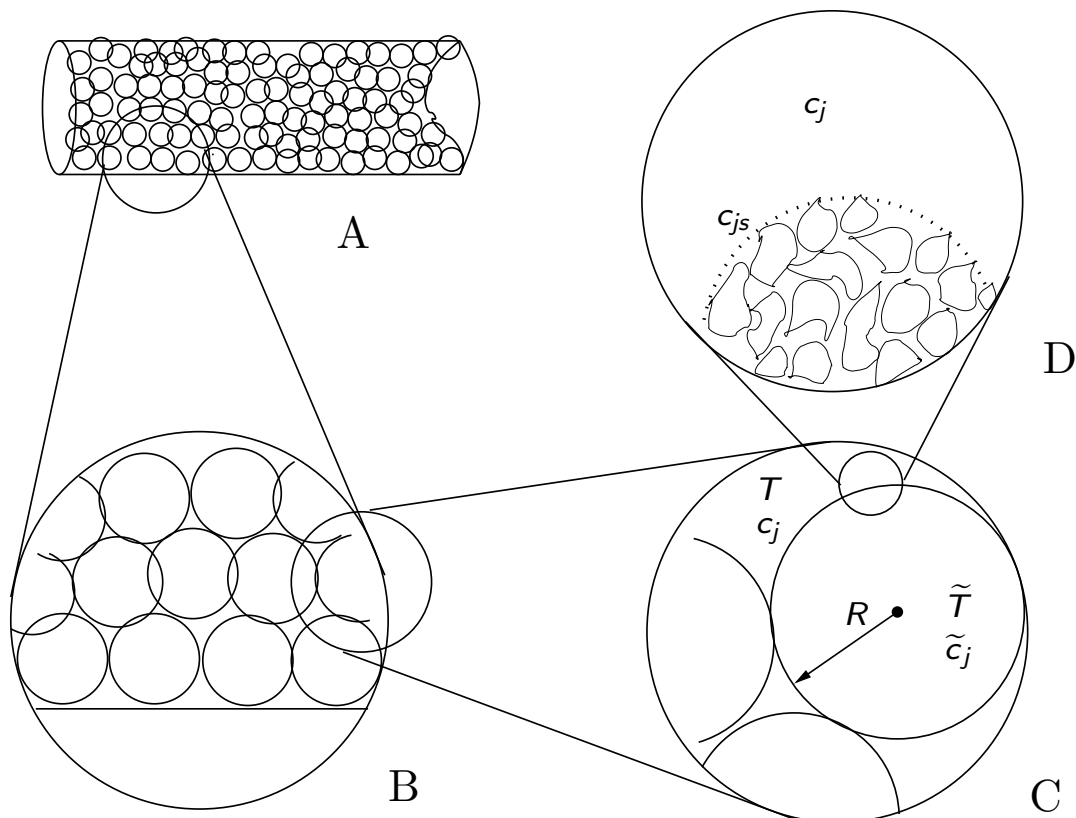
Figure 7.1: Expanded views of a fixed-bed reactor.
