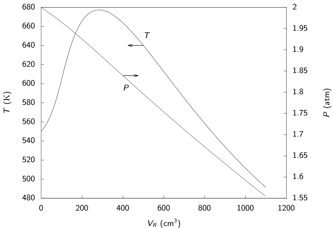
Figure 7.30: Fluid temperature and pressure versus reactor volume.
