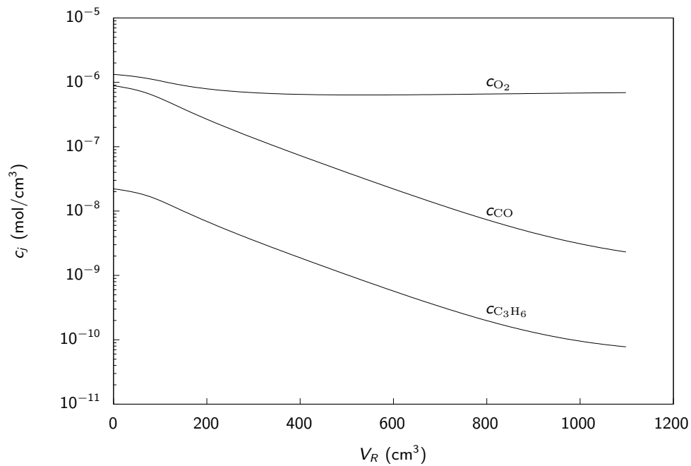
Figure 7.29: Fluid molar concentrations versus reactor volume.
