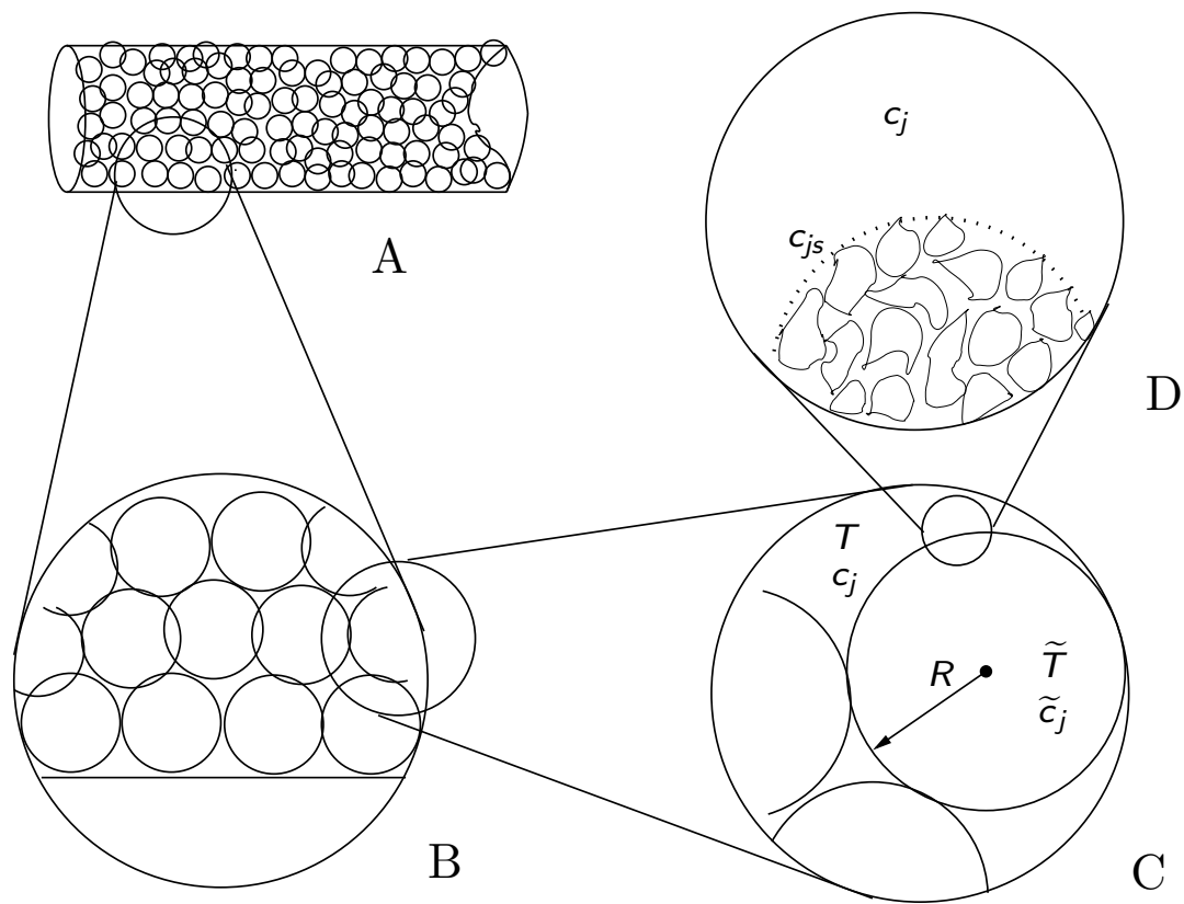
Figure: Expanded views of a fixed-bed reactor.
