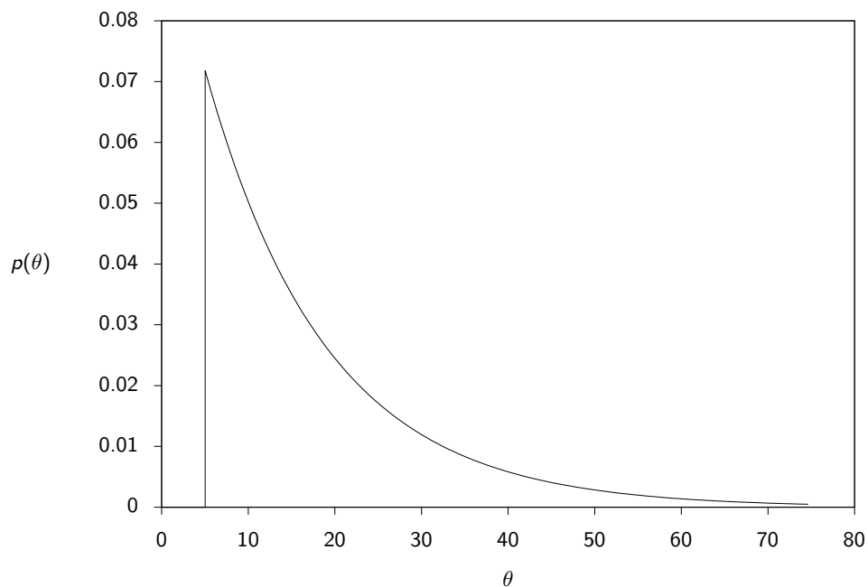
Figure 8.31: Residence-time distribution for the optimal reactor configuration.
