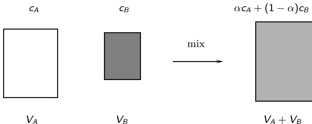
Figure 8.25: Two volume elements before and after mixing.
