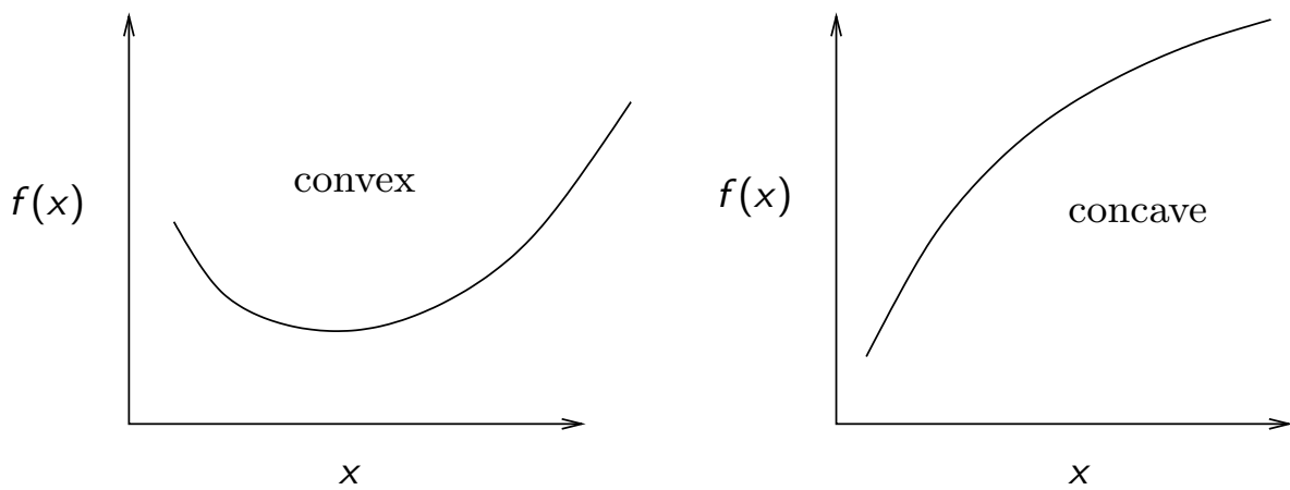
Figure 8.24: Differentiable convex and concave functions.
